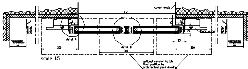
horizontal section B-B
